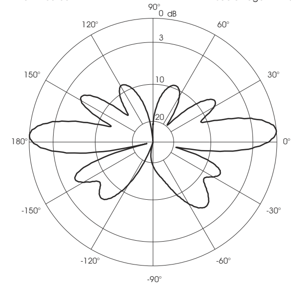
TYPICAL RADIATION PATTERN in E-plane at 920 MHz
